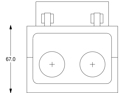
IP725/2H Brass Plate + 2 x 25mm Holes
